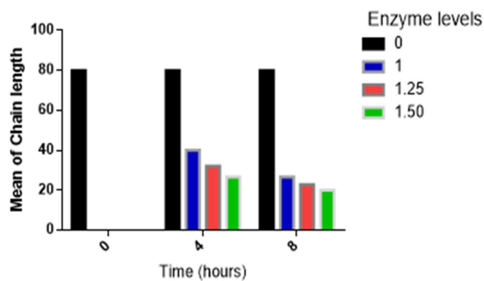
Figure 3. Calculated peptide chain length at different enzyme concentrations and incubation times
