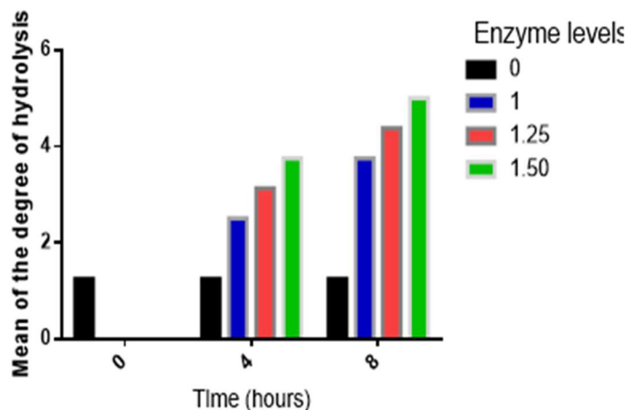
Figure 4. Degree of protein hydrolysis at different enzyme concentrations and incubation times
