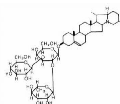
Figure 4. A typical saponin called solanine. Source: (36)
